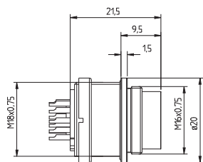
Solder connection
