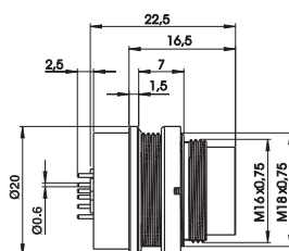
Dip solder connection
