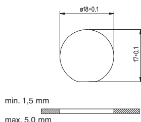
Installation dimensions
