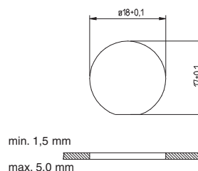
Installation dimensions
